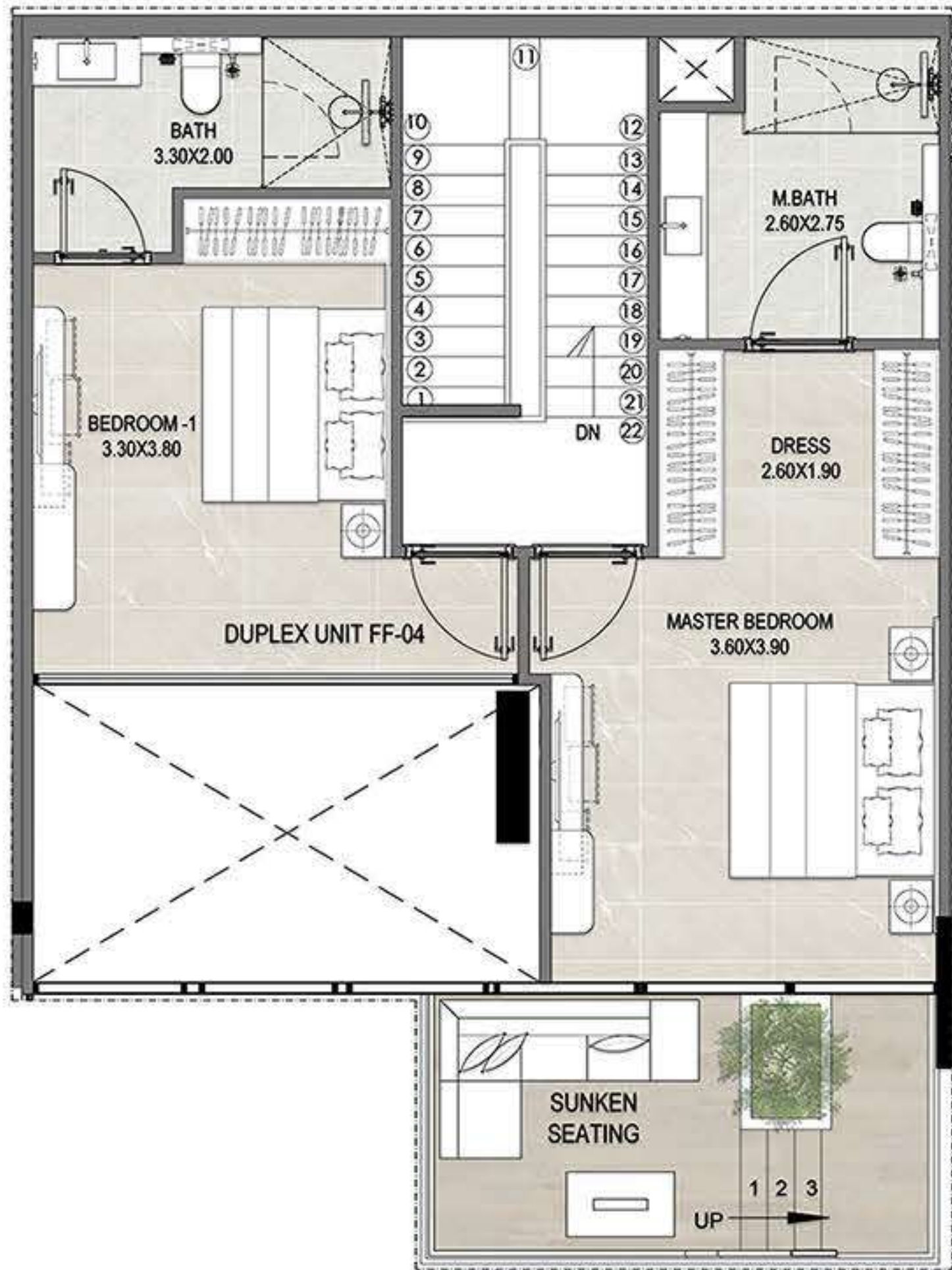
UPPER FLOOR
