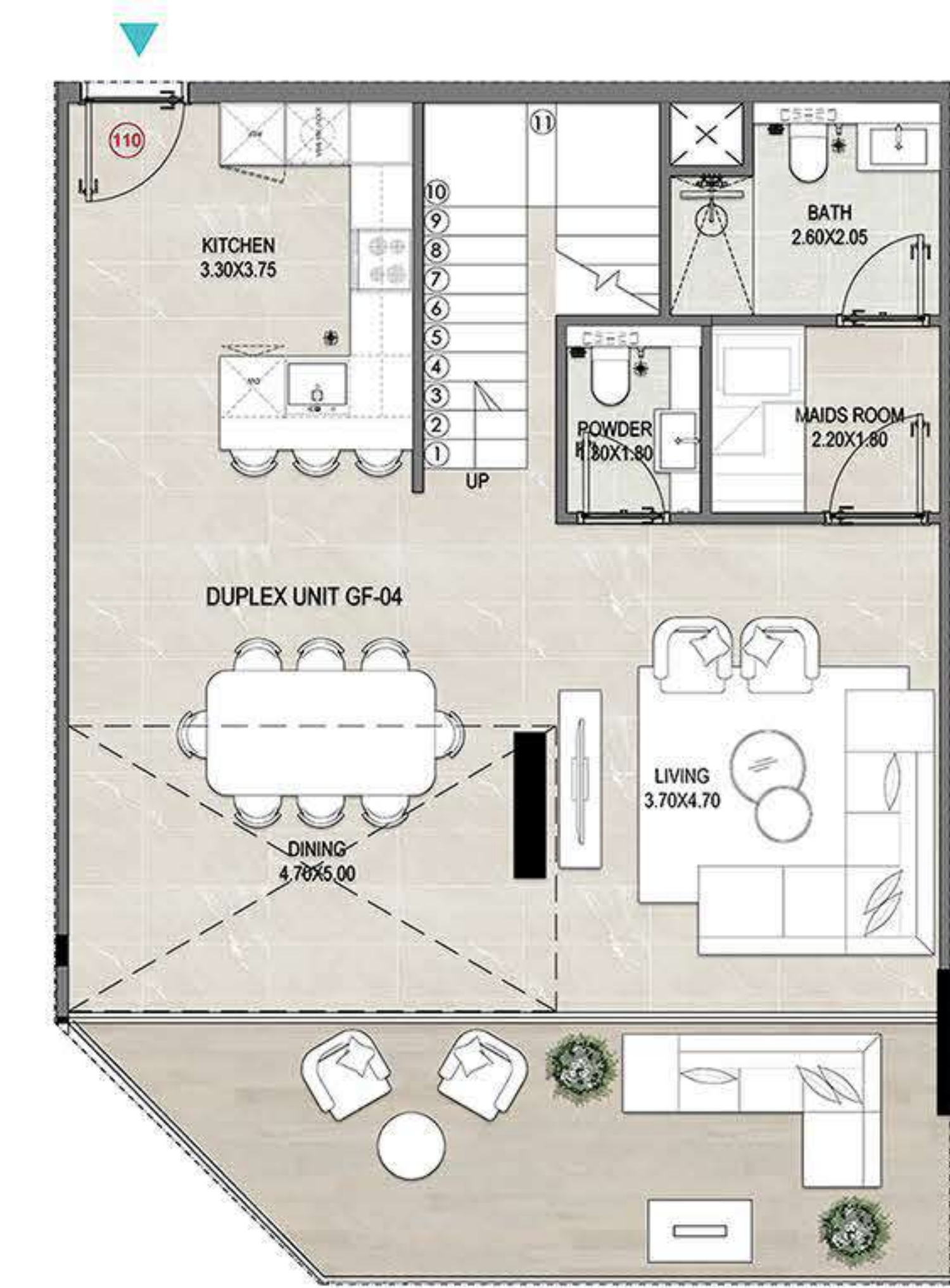
LOWER FLOOR
