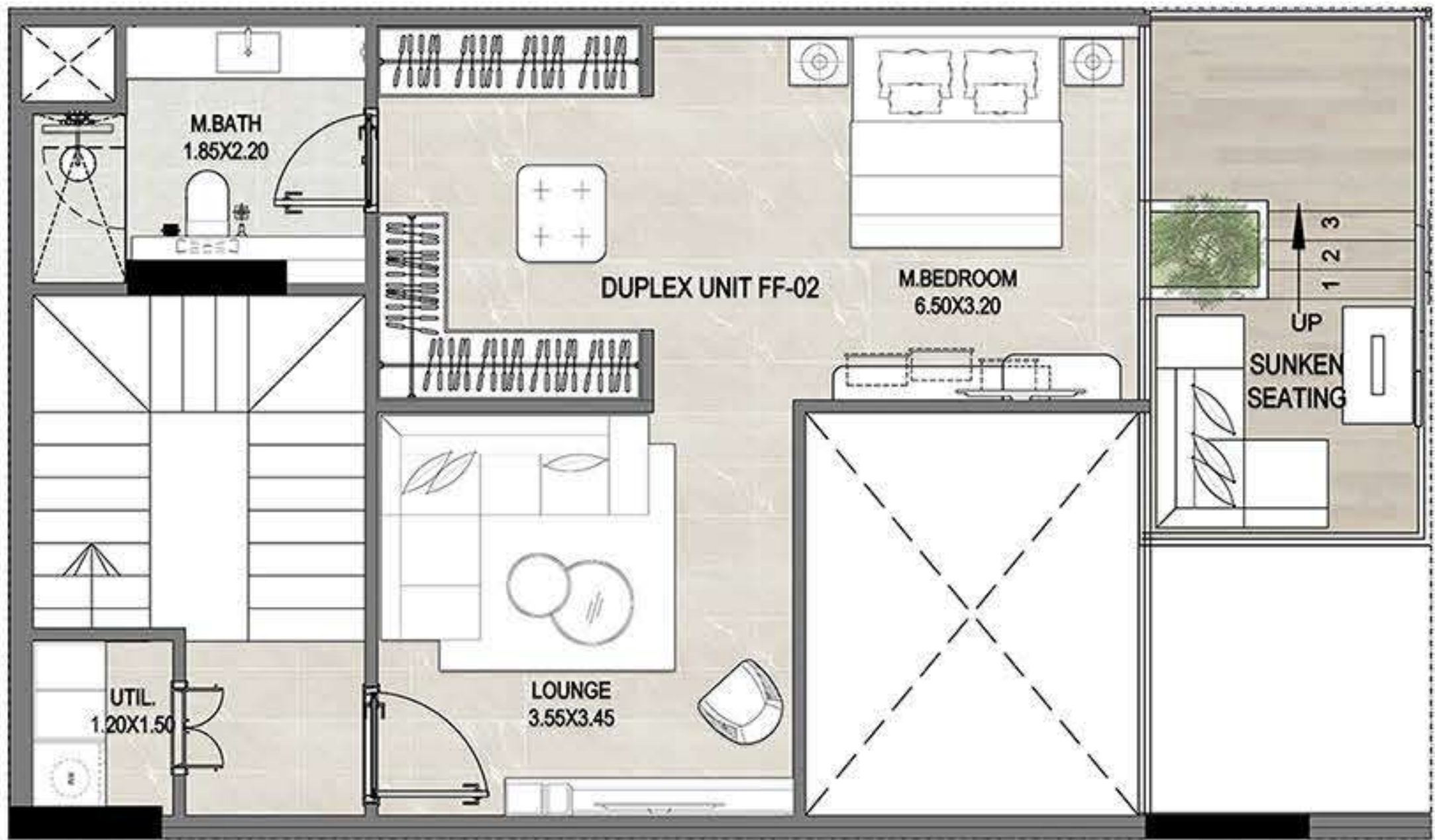
UPPER FLOOR
